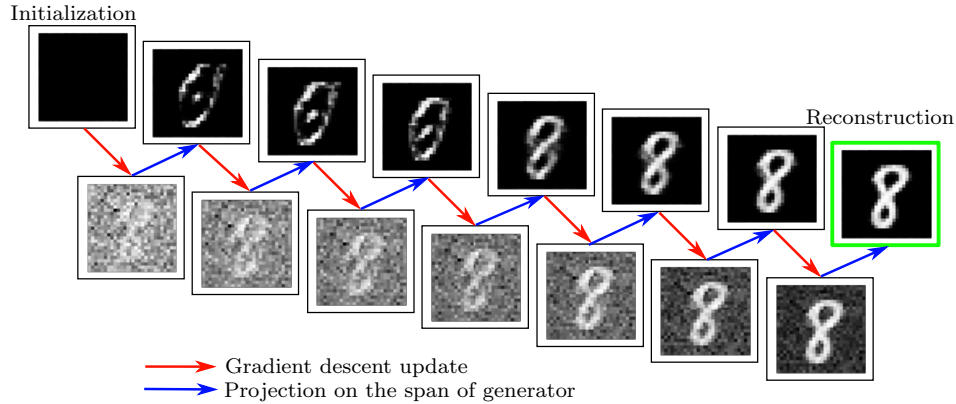
Figure 1.2 Illustration of our algorithm. Starting from a zero vector, we perform a gradient descent update step (red arrow) and projection step (blue arrow) alternatively to reach the final estimate.
