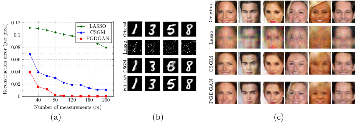
Figure 4.1 (a) Comparison of our algorithm (Alg. 1) with CSGM [5] and Lasso on MNIST; (b) Reconstruction results with m = 100 measurements; (c) Reconstruction results on celebA dataset with m = 1000 measurements.
